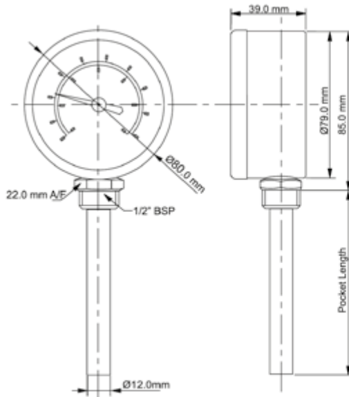
Dimensions: 80mm Dial thermometer - bottom entry
