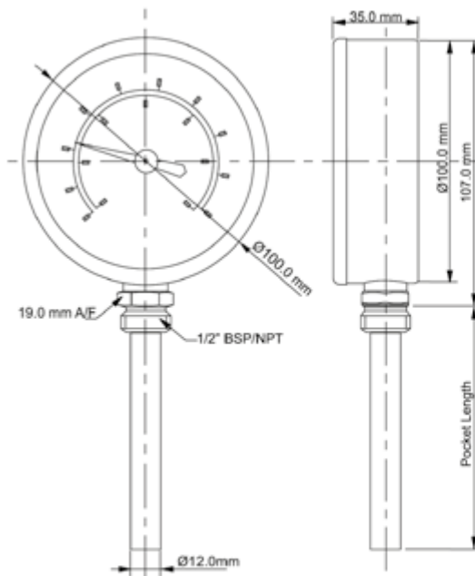
100mm Dial thermometer - bottom entry
