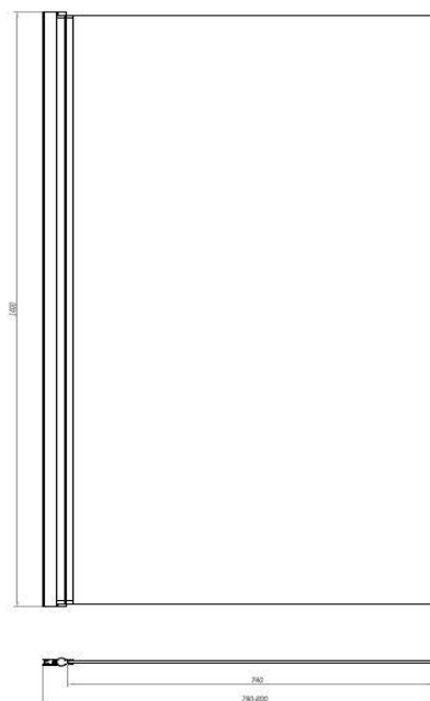
Square Bathscreen Panel
