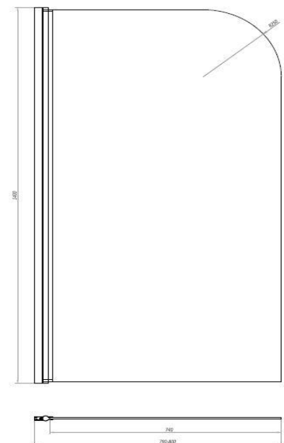
Radius Bathscreen Panel
