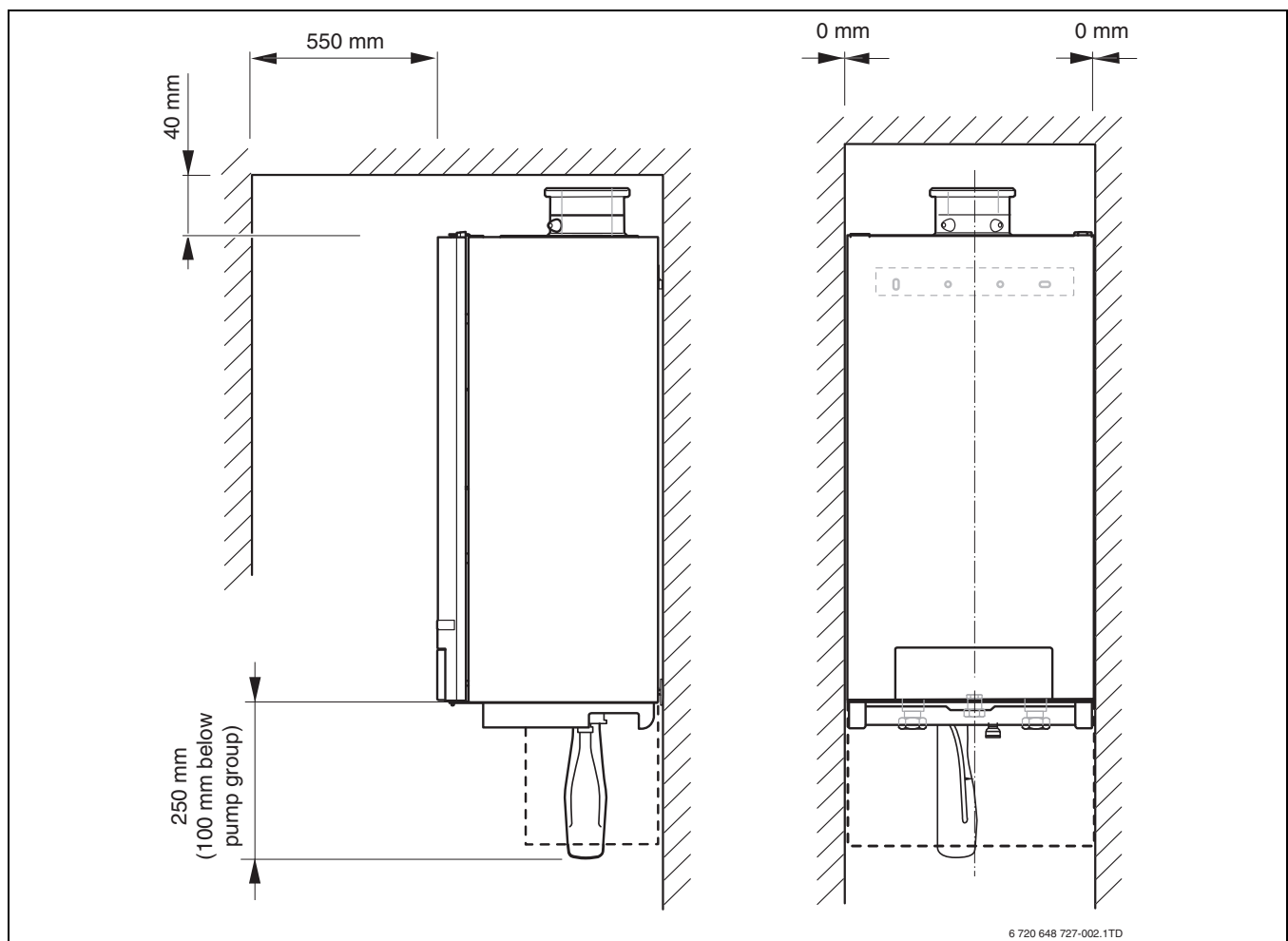
Fig. 2 Clearances
