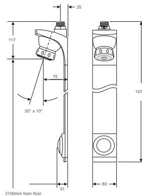
Dimensions (mm)
