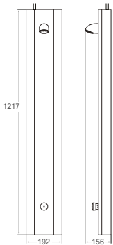
Dimensions (mm)
